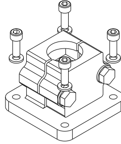
Description: Base clamp Ø30 Part number: 90.74.943
