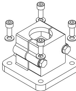
Description: Base clamp Ø40 Part number: 90.74.944
